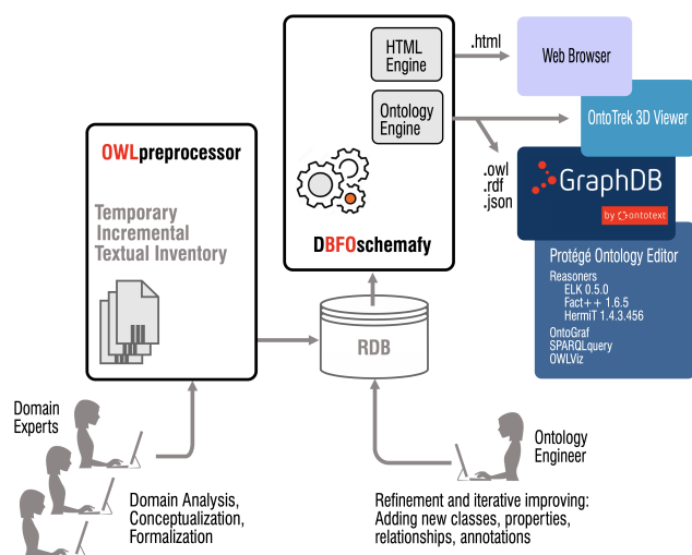
Figure 6: Development pipeline structure.
