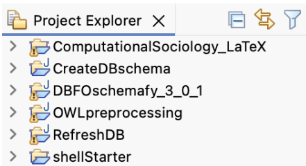
Figure 15: Eclipse projects.
